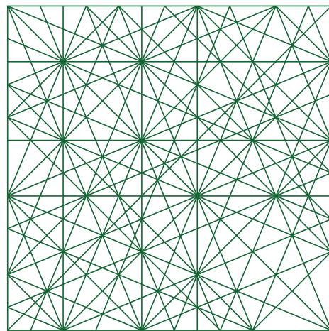
Figure 1: Maekawa-gami: 22.5^\circ grid.
